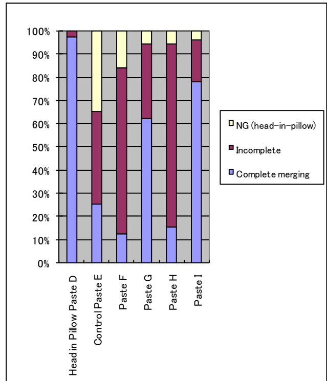
Figure 15: Solder joint formation of the different lead-free SnAgCu paste testing
