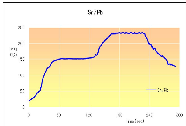
Figure 3: Reflow profile used to oxidize the tin-lead solder paste (Time over 183°C = 120 seconds)
