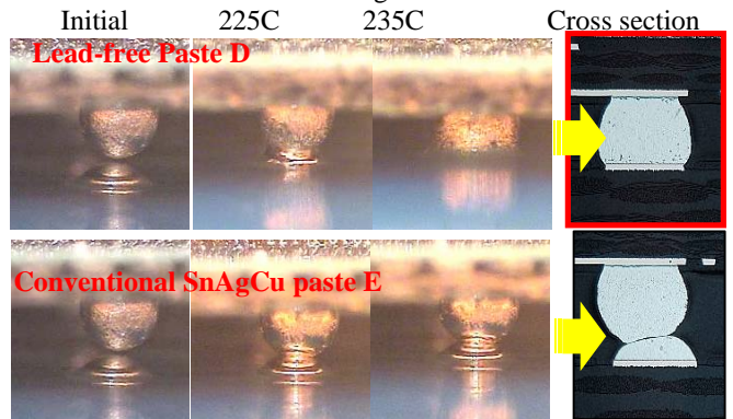
Figure 13: Observations in a reflow simulator for oxidized BGA/CSP components with Lead-free Head-in-Pillow SnAgCu Paste D versus the conventional SnAgCu paste
