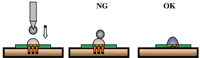
Figure 7: Diagram showing flux activation level evaluation
