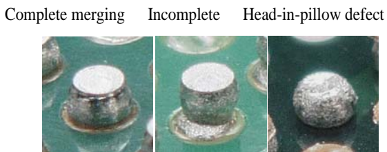
Figure 14: BGA Joint formation results for Lead-free Head-in-Pillow Paste D versus conventional SnAgCu paste E.
