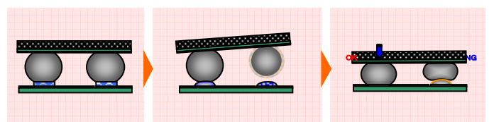
Figure 2: Head-in-pillow defect (Warpage, oxidization)
